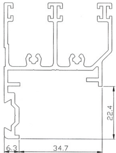
FULL SIZE SECTION THROUGH OUTER FRAME
