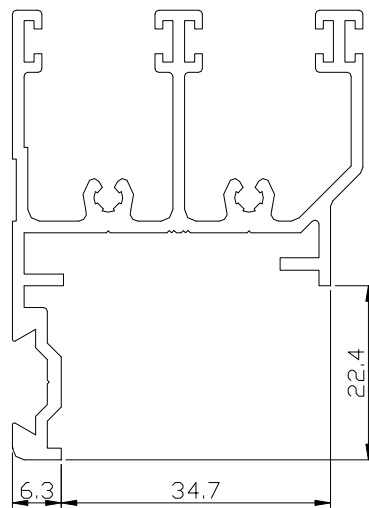
FULL SIZE SECTION THROUGH OUTER FRAME
