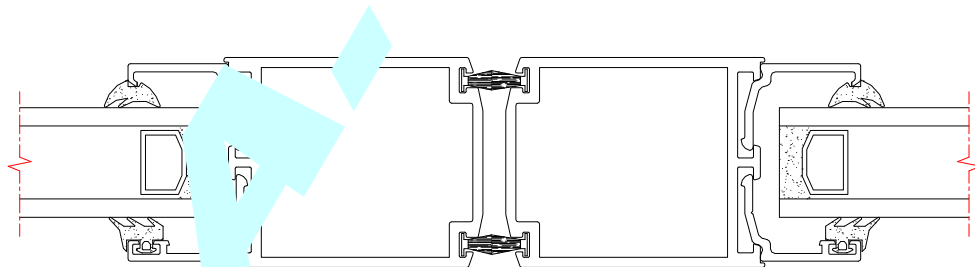
DETAIL OF DOUBLE DOOR MEETING STILE
