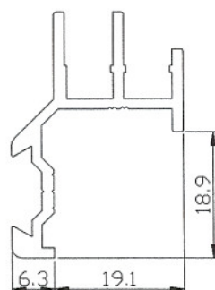
FULL SIZE SECTION THROUGH OUTER FRAME
